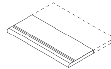
Marche Sand_Stone Granito Beirão Peldaño Sand_Stone Granito Beirão 78x58x3,5cm
